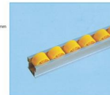
Aluminium slide way SQ-44B Aluminium framework ( W*H): 44mm* 38mm Total height( include wheel): 48mm ABS roller : φ38*25mm Roller shaft : 45# Galvanization steel Distance of roller shaft : 45mm Quantity : 22pcs/meter Workload of single roller shaft : 20kg Workload of each meter : 80kg
