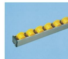
Aluminium slide way SQ-41B Aluminium framework ( W*H): 41mm* 35mm Total height( include wheel): 42.5mm ABS roller : φ38* 28*25mm Roller shaft : 45# Galvanization steel Distance of roller shaft : 45mm , 60mm Quantity : 22pcs,16pcs/meter Workload of single roller shaft : 10kg Workload of each meter : 100kg
