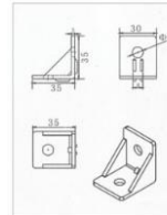
Aluminum corner connector 3
