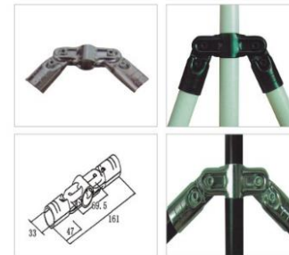
No. : HJ-12P/HJ-12D Form : H-6P/D*4+H-14P/D*2+M6-25*4pcs
