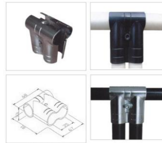
No. : HJ-9P/HJ-9D Form : H-10P/D*2+M6-25*1pcs
