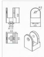
Aluminum corner connector 7
