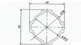
Name: Aluminium tube(big) Material: 6063-T5 (Surface oxidation spray with white sand) P/N: T3-AL4319 Standard length: 4m/pcs Weight: 0.72kg/m Thickness: 1.9mm
