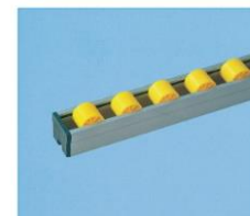
Aluminium slide way SQ-41B Aluminium framework ( W*H): 41mm* 35mm Total height( include wheel): 42.5mm ABS roller : φ28*25mm Roller shaft : 45# Galvanization steel Distance of roller shaft : 30mm,45mm,60mm Quantity : 33pcs , 22pcs , 16pcs/meter Workload of single roller shaft : 10kg Workload of each meter : 100kg
