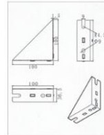
Aluminum corner connector 8
