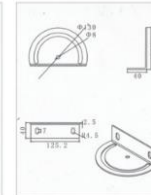
Aluminum corner connector 9
