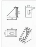
Aluminum corner connector 2
