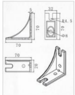
Aluminum corner connector 6
