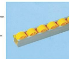
Aluminium slide way SQ-44A Aluminium framework ( W*H): 44mm* 33mm Total height( include wheel): 40mm ABS roller : φ38*25mm Roller shaft : 45# Galvanization steel Distance of roller shaft : 45mm Quantity : 22pcs/meter Workload of single roller shaft : 20kg Workload of each meter : 80kg
