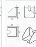
Aluminum corner connector 5
