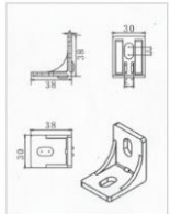
Aluminum corner connector 1
