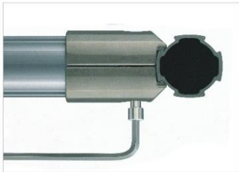
Name: Aluminium tube P/N: T3-AL2812/T3-AL2817 Material: 6063-T5(surface oxidation spray with white sand) Standard length: 4m/pcs Weight: 0.38kg/m (T=1.2mm) 0.42kg/m (T=1.7mm)
