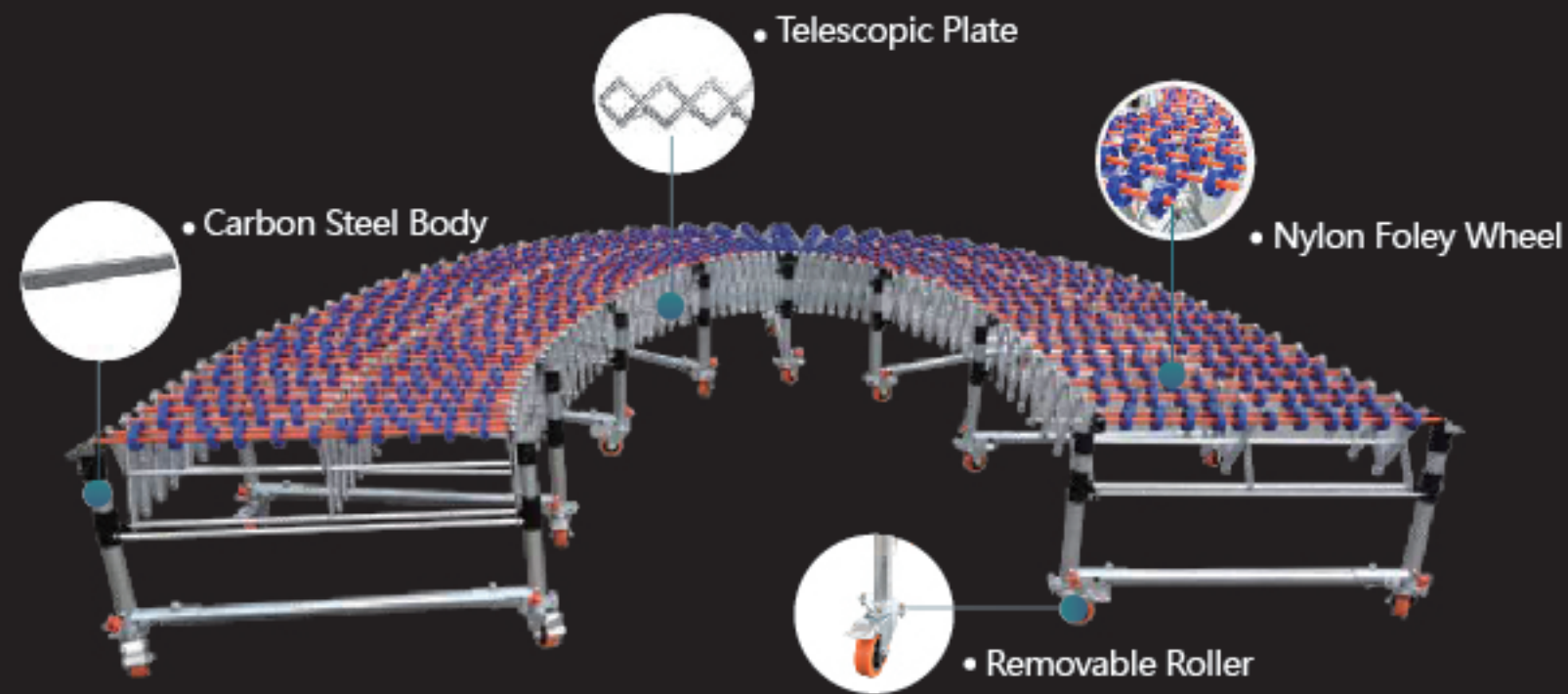
360-degree Rotatable Unpowered Loading And Unloading Conveyor
